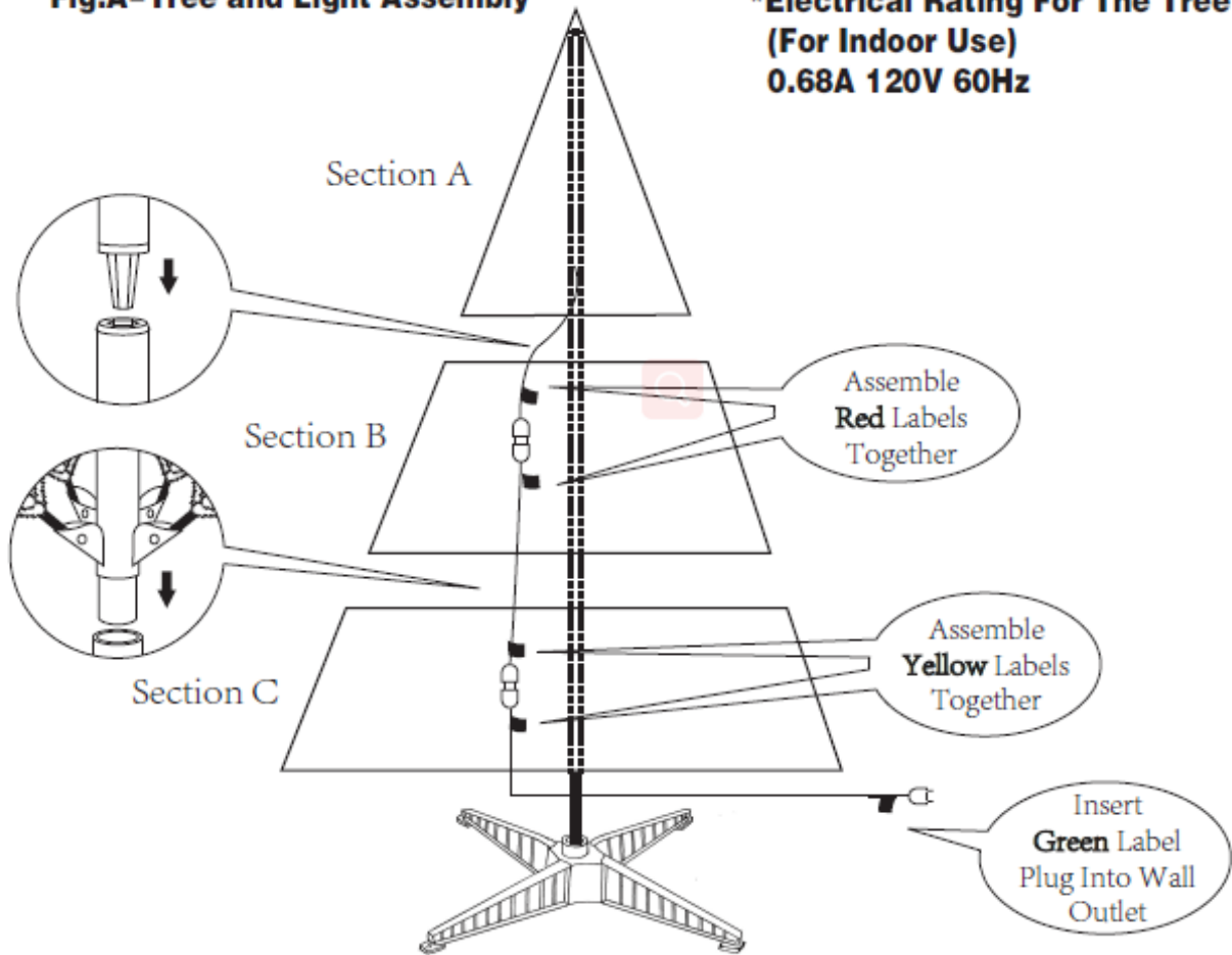
Fig.A-Tree and Light Assembly
